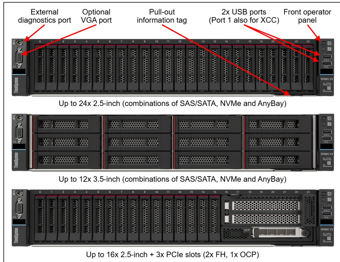
Figure 2. Front view of the ThinkSystem SR665 V3
