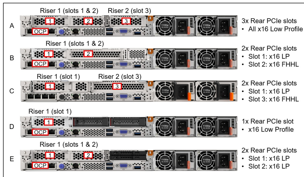
Figure 14. SR630 V3 rear slot configurations
