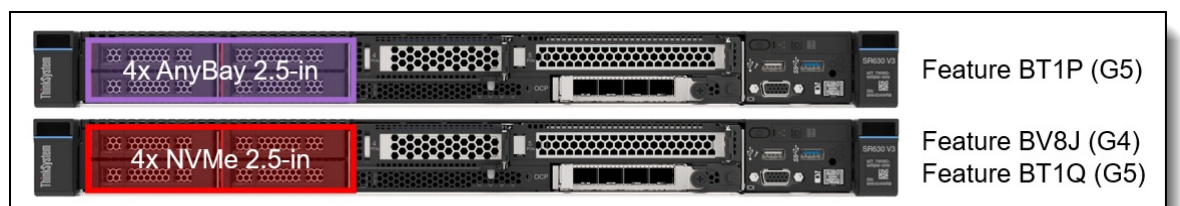
Figure 11. SR630 V3 front drive bay configurations - 2.5-inch drive bays with front PCIe slot support
