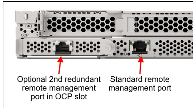
Figure 23. SR630 V3 with the Redundant System Management Port Adapter installed
