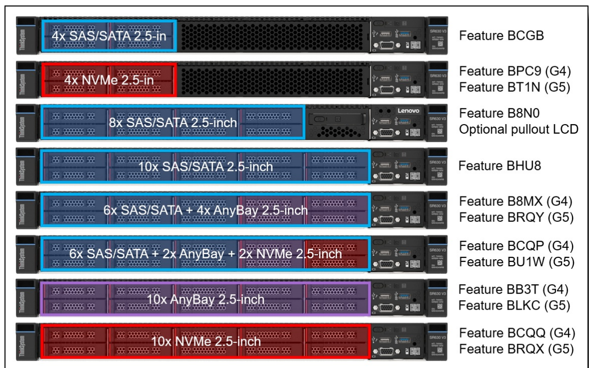
Figure 10. SR630 V3 front drive bay configurations - 2.5-inch drive bays without front PCIe slot support
