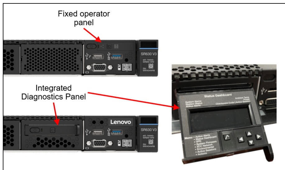
Figure 21. Operator panel choices for the 8x 2.5-inch drive bay configuration
