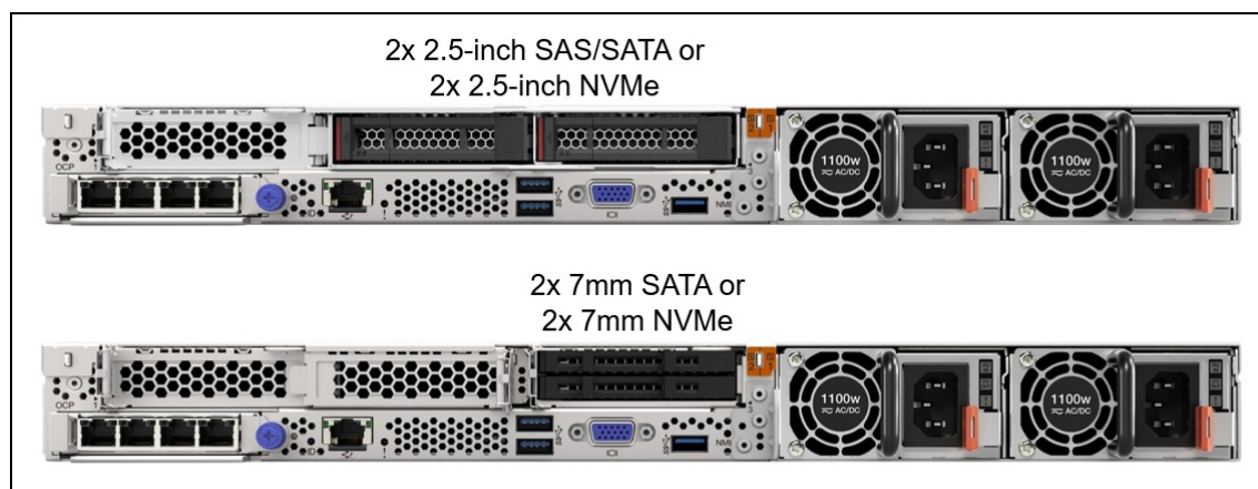
Figure 12. Rear drive bay configurations
