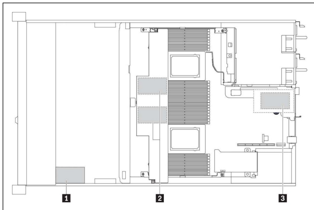
Figure 17. Potential locations of all supercaps in the SR630 V3 (2.5-inch drive configuration and standard heatsinks)
