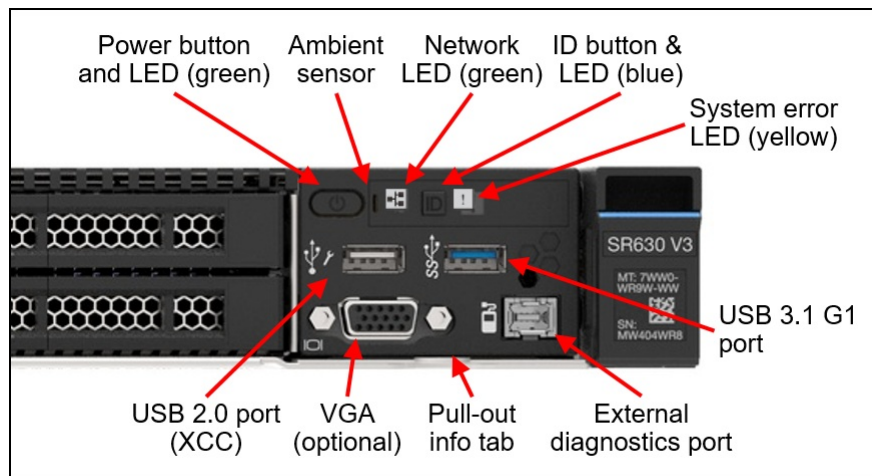
Figure 20. SR630 V3 Front operator panel
