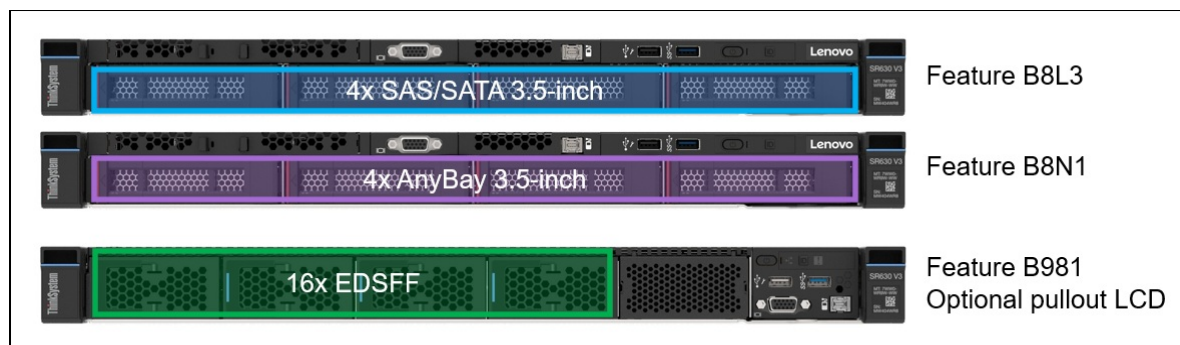
Figure 9. SR630 V3 front drive bay configurations - 3.5-inch and EDSFF drive bays
